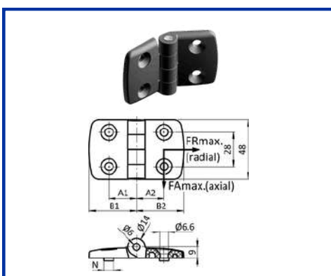
STANDARD HINGE 40 X 40 PLASTIC
