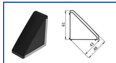
END CAP FOR GUSSET 45 X 90
