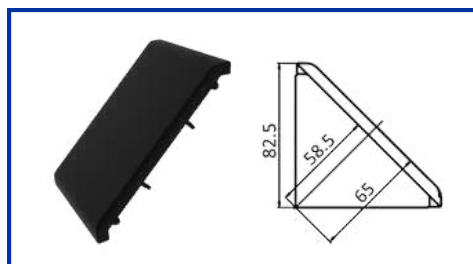
END CAP FOR GUSSET 80 X 80
