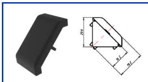
END CAP FOR GUSSET 45 X 45
