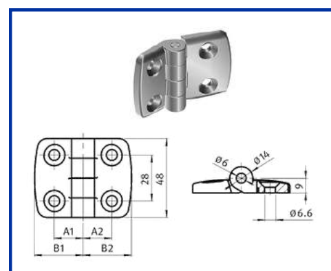
ALUMINUM COMBI HINGE 30
