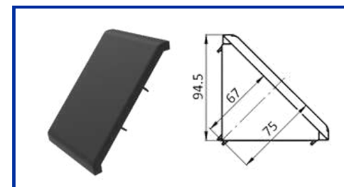
END CAP FOR GUSSET 90 X 90
