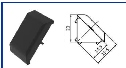
END CAP FOR GUSSET 40 X 40
