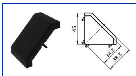
END CAP FOR GUSSET 80 X 80
