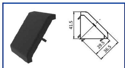
END CAP FOR GUSSET 60 X 60
