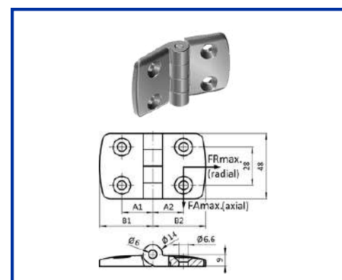
ALUMINUM COMBI HINGE 40
